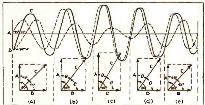
Fig. 6. Advance in phase on one side of audio wave.
