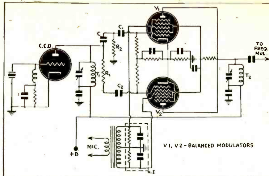
Fig. 4—This simplification of the conventional FM circuit dispenses with the mixer tube of Fig. 1.
