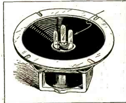
Fig. 4—Shims in position for centering cone.
